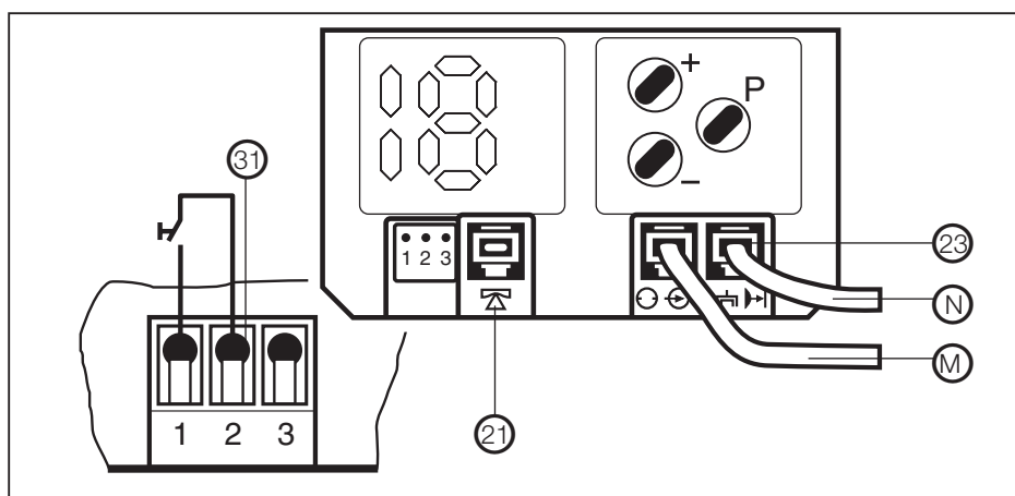
Abb. 8: Anschlüsse
